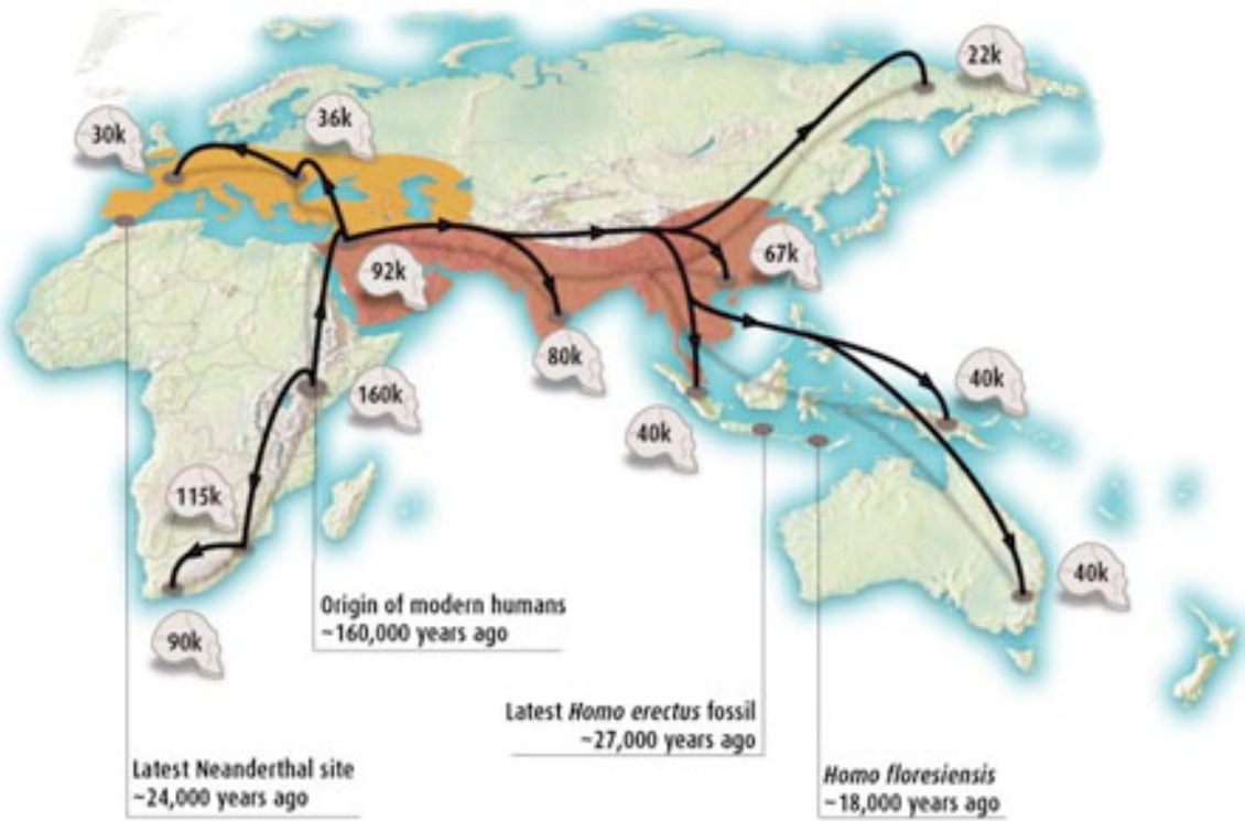
● Neanderthal range -130,000 - 30,000 years ago ● Range of Homo erectus in Asia -1.9 million - 30,000 years ago
